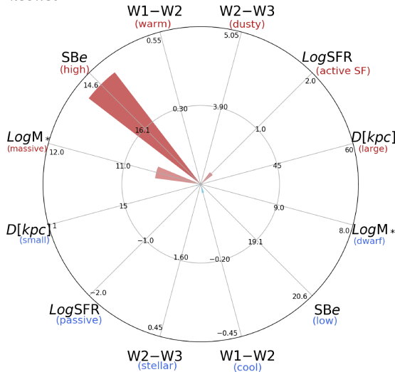
NGC4736
