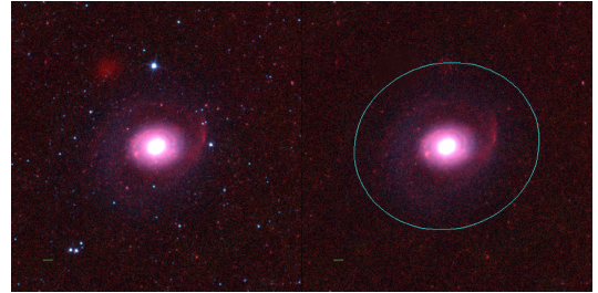
NGC4736
