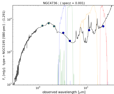
NGC4736
