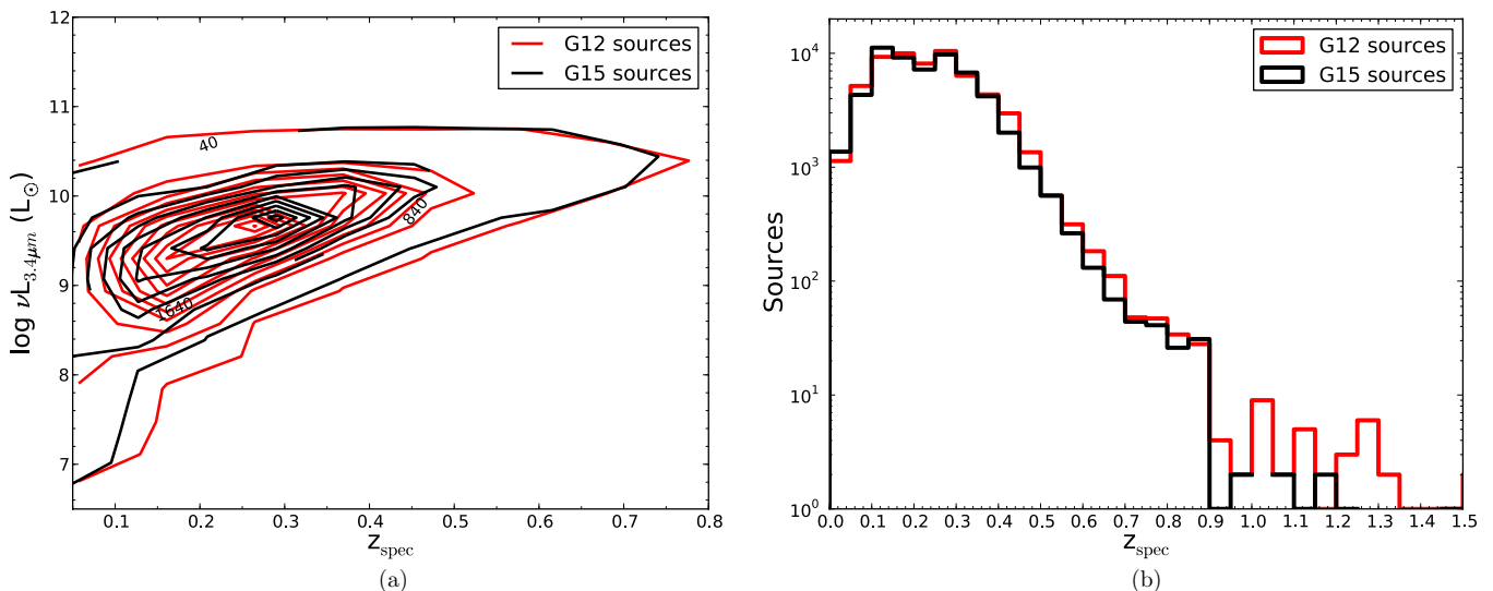
Figure 4. (a) The 3.4 \mu\text{m} luminosity density ( \nu L_\nu ) distribution of sources in the two GAMA fields as a function of redshift. The number distribution as a function of redshift is shown in panel (b).
