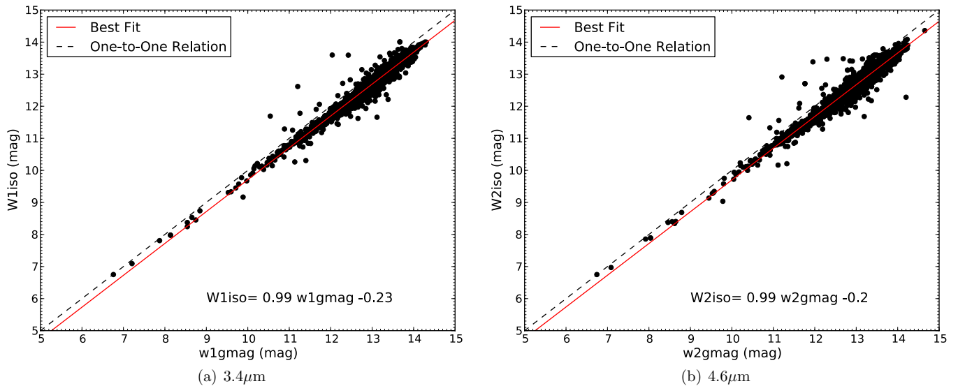
Figure 2. Comparisons of 1\sigma isophotal photometry ( W_{\star iso} ) and the 2MASS XSC-derived scaled aperture ( w_{\star gmag} ) photometry for resolved sources in the G12 and G15 fields. See Figure 20 for versions plotted as a function of w_{\star gmag} .
