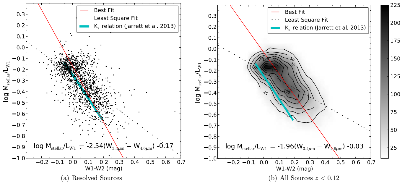
Figure 6. 3.4\ \mu\text{m} mass-to-light ratio plotted as a function of W1-W2 (Vega) color for (a) resolved sources and (b) all sources in G12 and G15. The larger volume sample shows a shift to more active galaxies with “warmer” W1-W2 colors.
