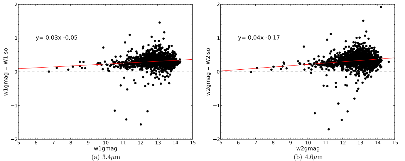
Figure 20. Comparison of w\star gmag and W\star iso photometry as a function of w\star gmag . (A color version of this figure is available in the online journal.)
