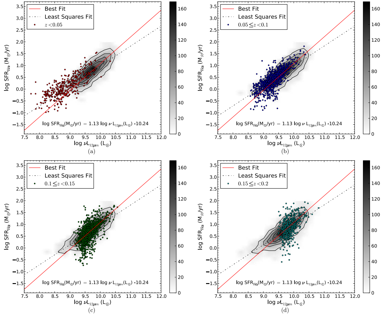
Figure 11. \text{H}\alpha -derived star formation rates as a function of \nu L_{12\mu\text{m}} luminosity for redshift slices of 0.05 between 0 < z < 0.2 overplotted on the full distribution from Figure 9.
