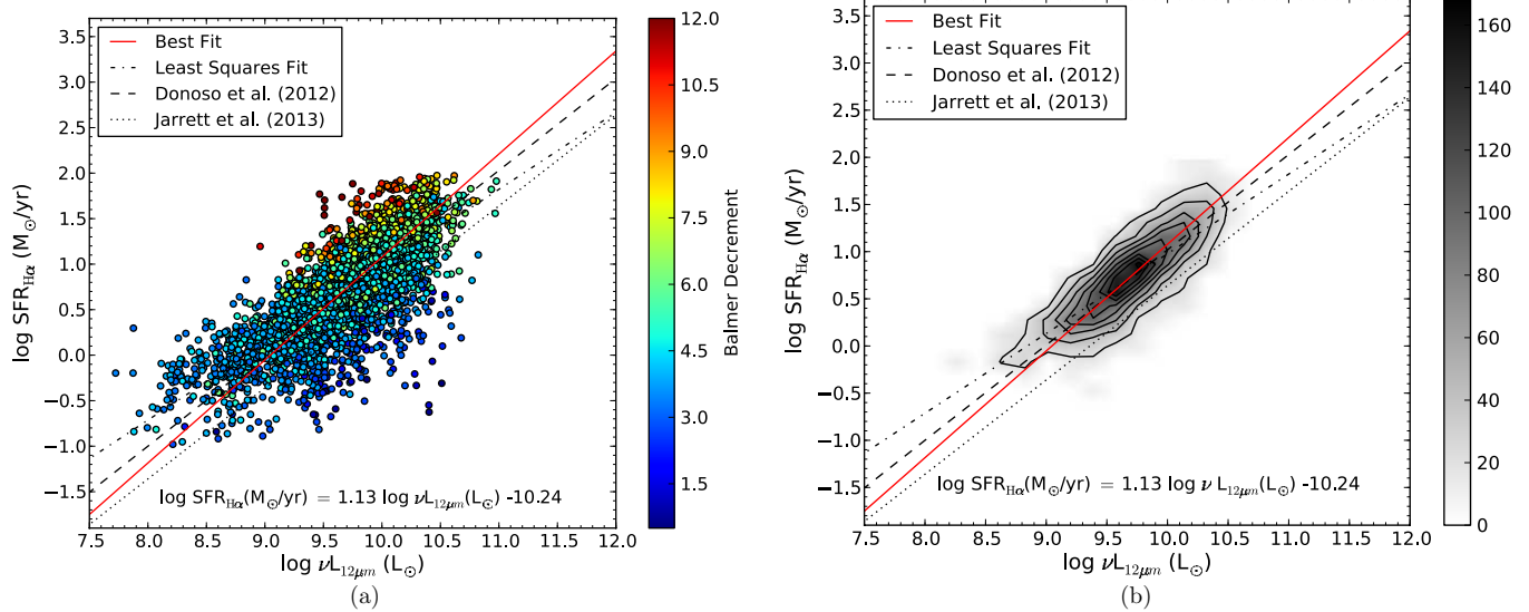
Figure 10. H\alpha -derived star formation rates as a function of \nu L_{12\mu m} luminosity color-coded by Balmer decrement in panels (a) and (b) shown as a contour and density plot.
