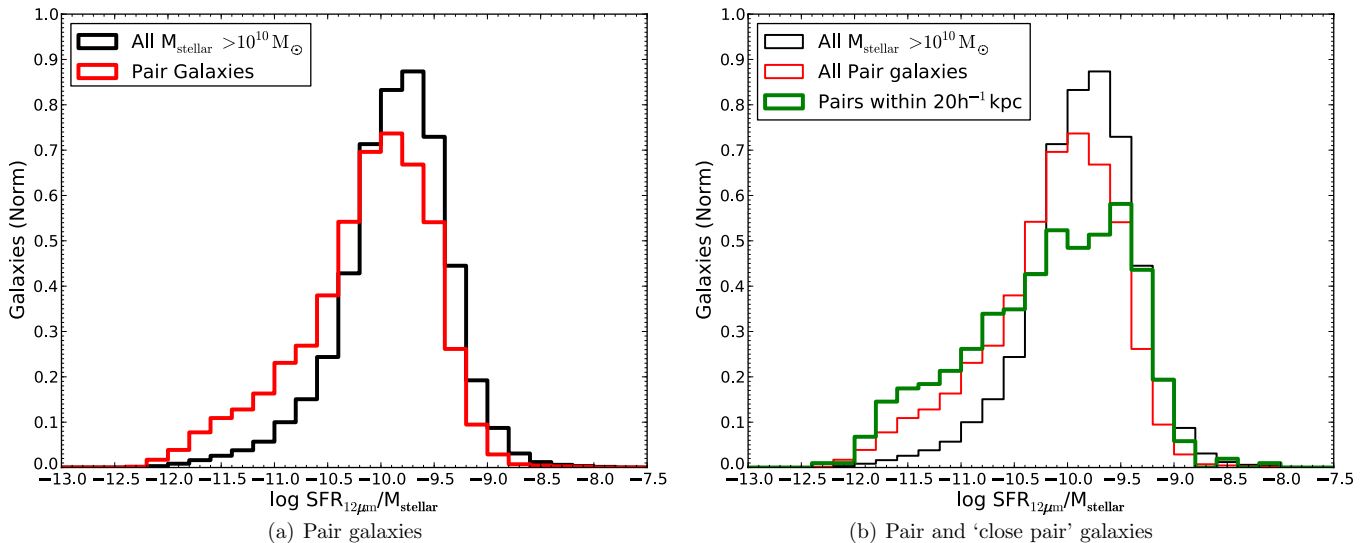
Figure 14. Specific star formation rate normalized distribution of galaxies with stellar masses > 10^{10} M_\odot and the subsets that reside within a pair and a close pair (separation < 20 h^{-1} \text{kpc} ).
